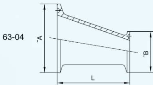
32-14MP Eccentric Reducer
