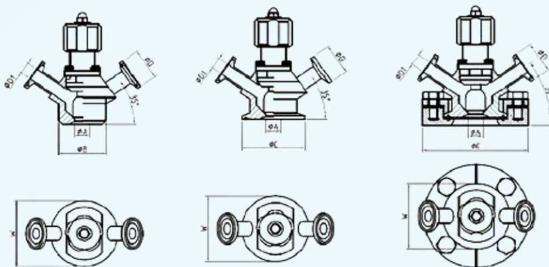
Fig. 1. Dimensions - valve.
